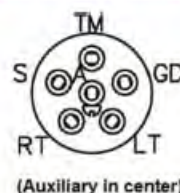
6-POLE PLUG
