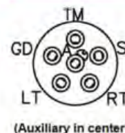
6-POLE SOCKET
